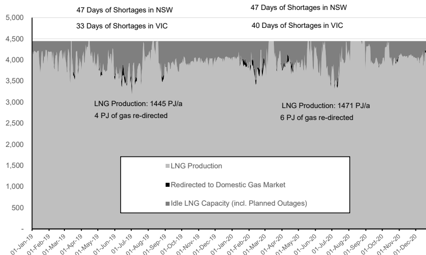
Figure 12: LNG fleet operations - 'no new pumped hydro' scenario Aggregate Gas Demand (TJ/d)
