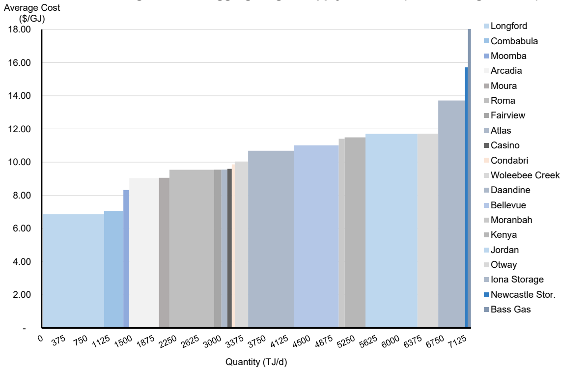
Figure 7: Aggregate gas supply function (east coast gas fields)
