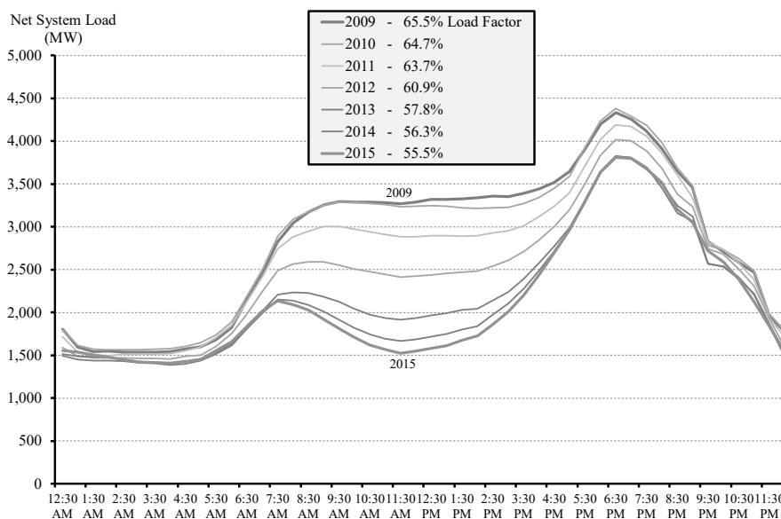
Figure 5: Distribution Network 'Average Net System Load Profile'
